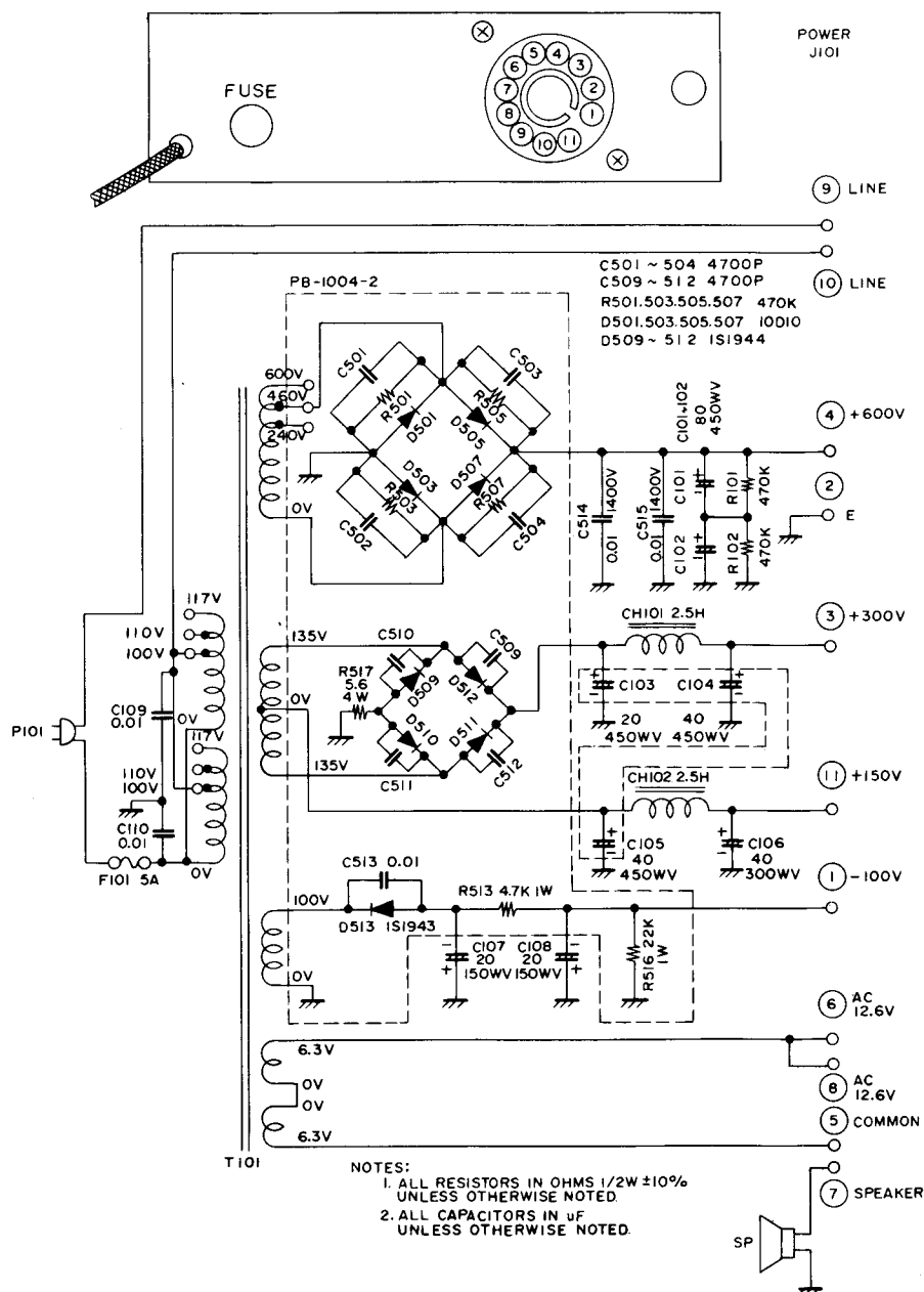
POWER SUPPLY
