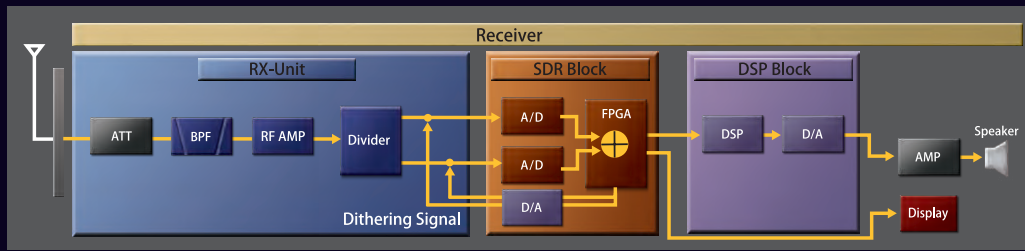
Receiver Block Diagram
