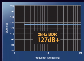
14MHz帯 BDR (Blocking Dynamic Range)
