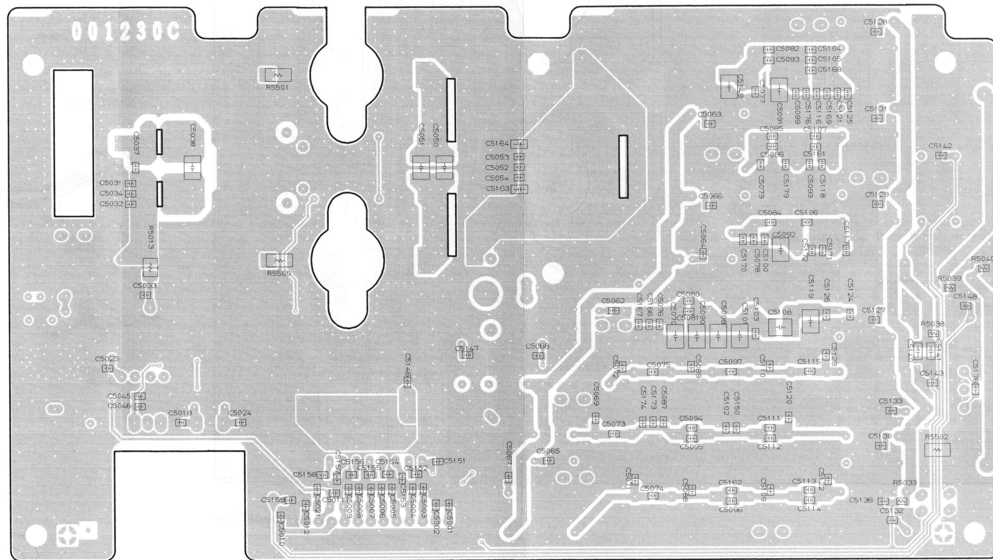
Chip Side
