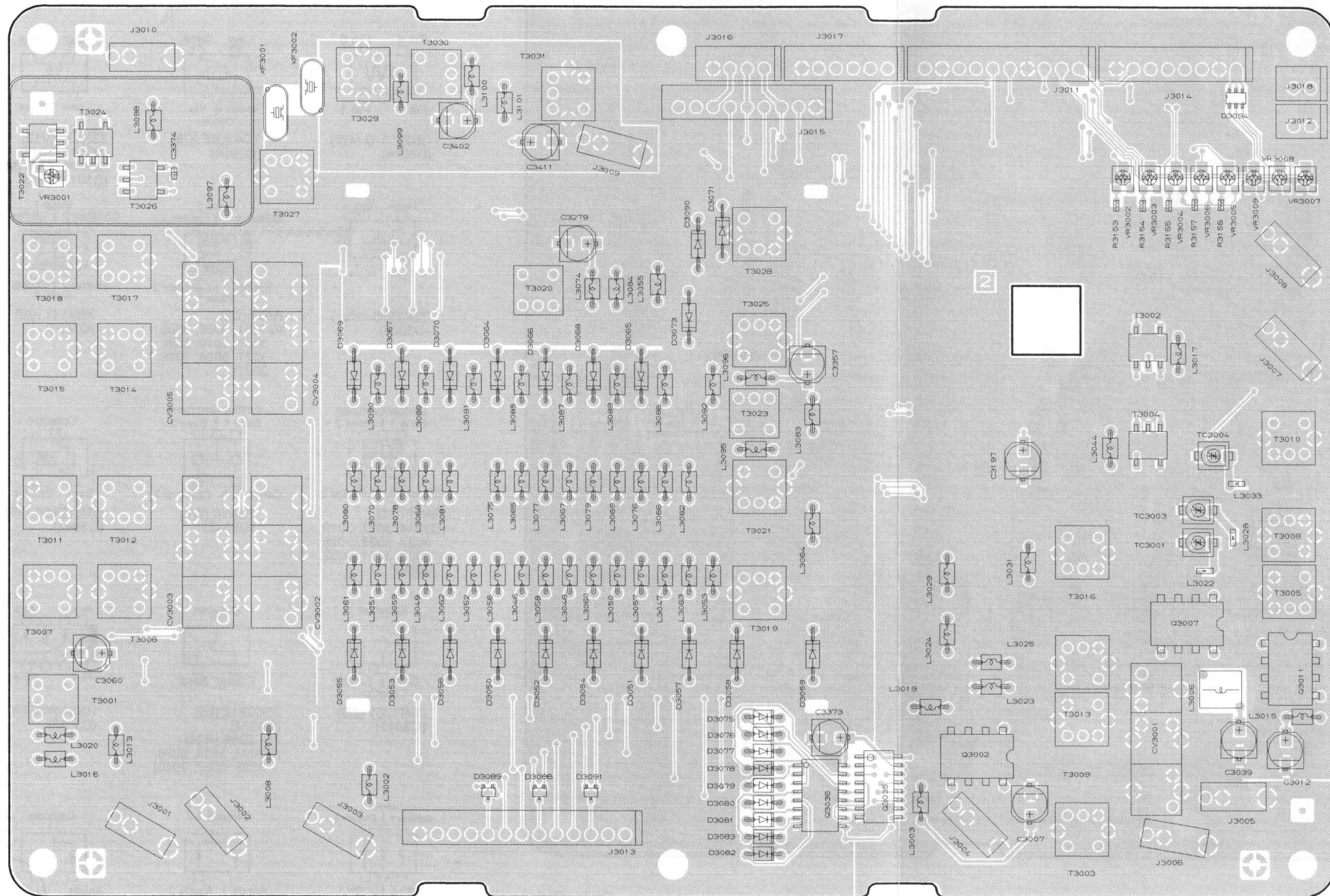
Component Side
