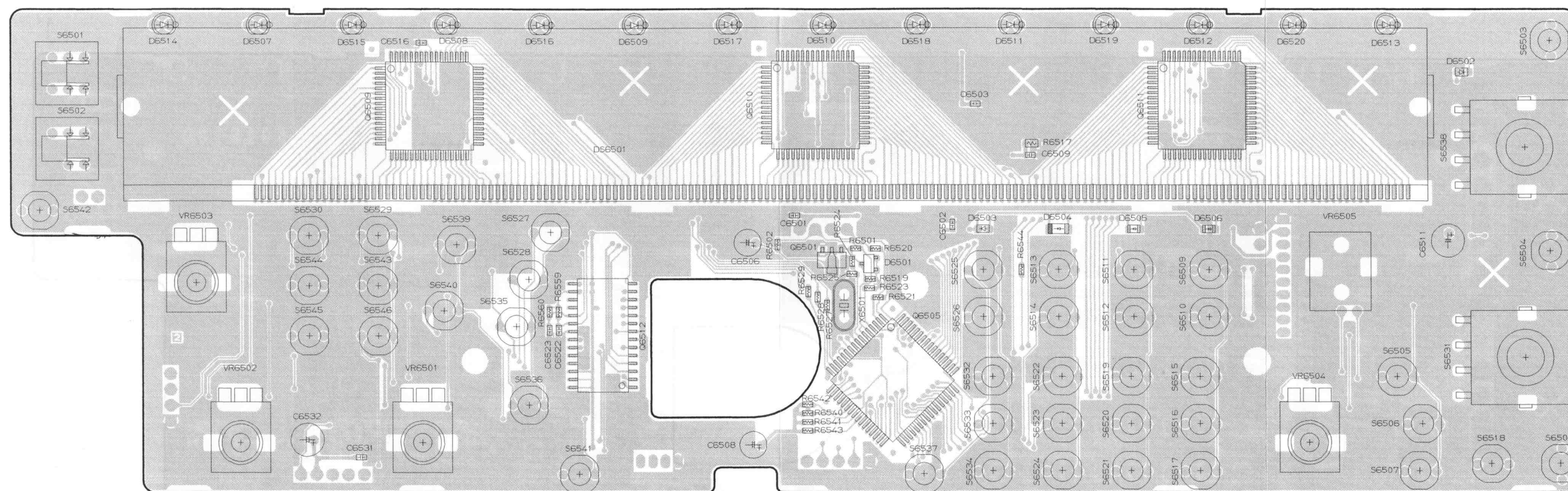
Component Side
