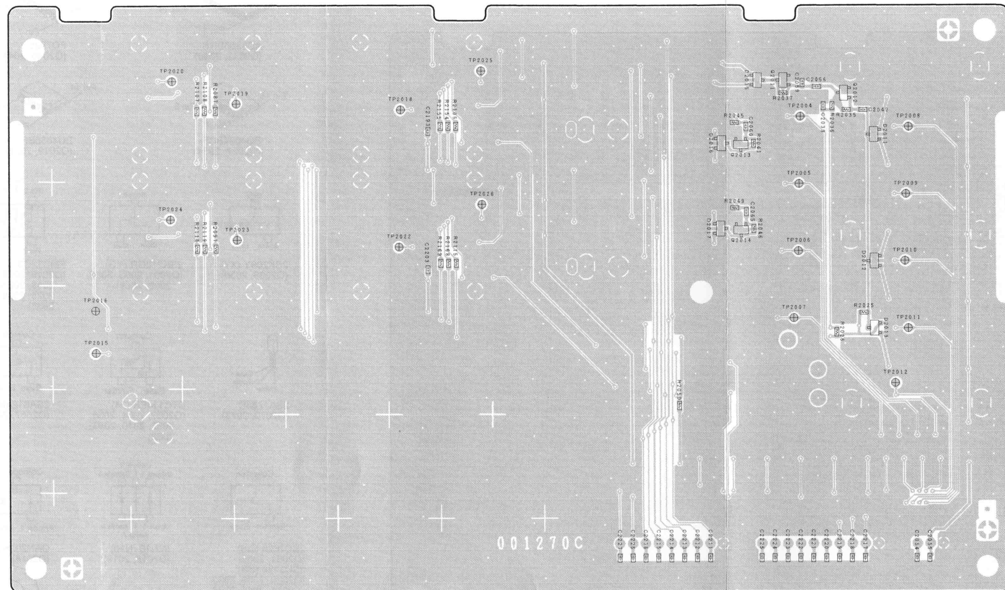
Chip Side
