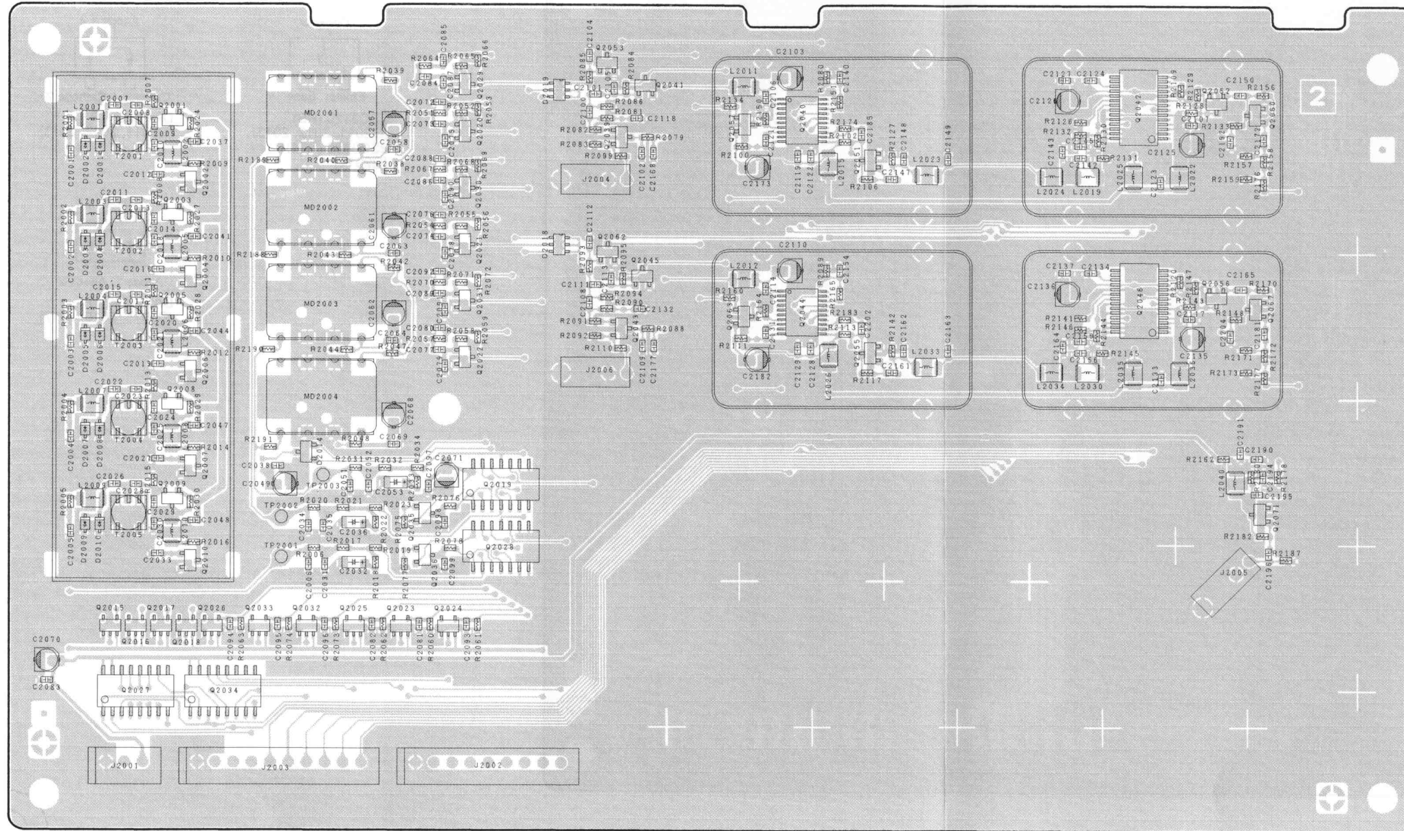
Component Side
