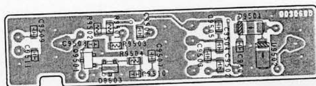
Chip Side
