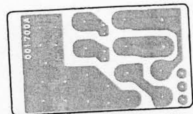
Solder Side
