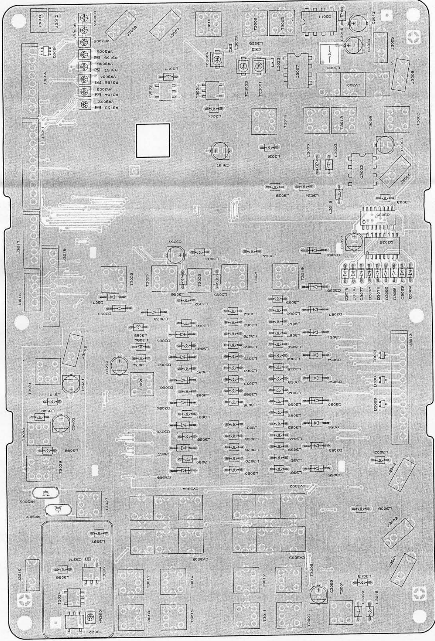
Component Side
