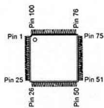
TMS320C203PZ57 (Q6012)
