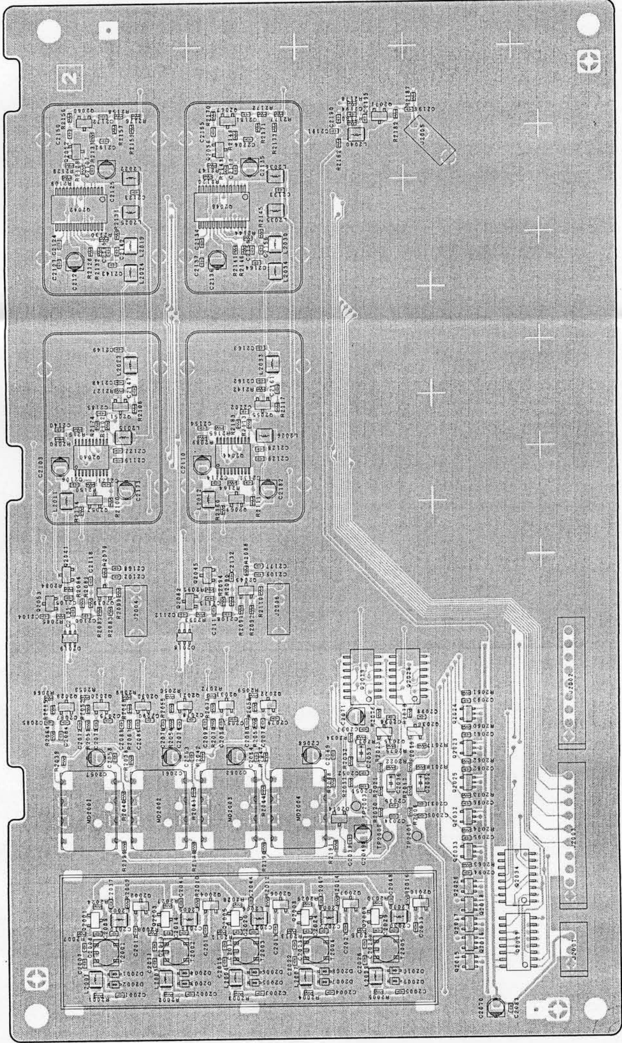
Component Side
