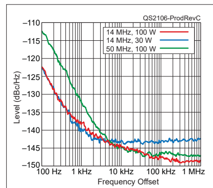
Figure C — The spectral display of the Yaesu FTdx10 transmitter output during phase-noise testing. Power output is 100 W on the 14 MHz band (red trace), 30 W on the 14 MHz band (blue trace), and 100 W on the 50 MHz band (green trace). The carrier, off the left edge of the plot, is not shown. This plot shows phase noise 100 Hz to 1 MHz from the carrier. The reference level is -110 dBc/Hz, and the vertical scale is 5 dB per division.
