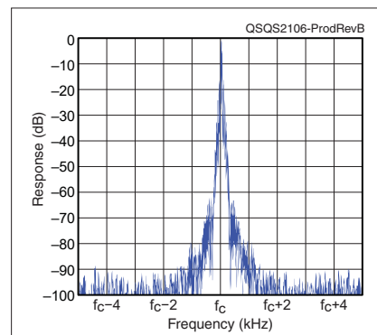
Figure B — The spectral display of the Yaesu FTdx10 transmitter during keying sideband testing. Equivalent keying speed is 60 WPM using external keying and the default 6-millisecond rise time setting. Spectrum analyzer resolution bandwidth is 10 Hz, and the sweep time is 30 seconds. The transmitter was being operated at 100 W PEP output on the 14 MHz band, and this plot shows the transmitter output ±5 kHz from the carrier. The reference level is 0 dBc, and the vertical scale is in decibels.
