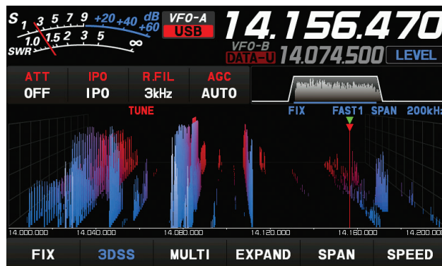
Figure 3 — The FTDX10's fascinating 3DSS display mode represents signals as receding spikes in constant motion. You can also opt for a more traditional waterfall display.
