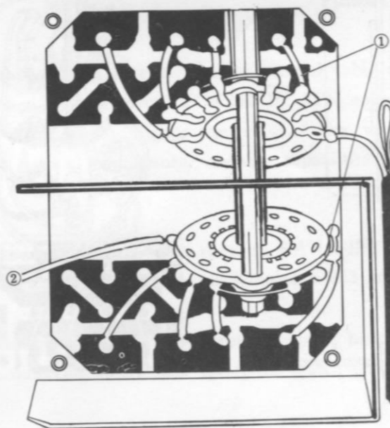
BOTTOM VIEW
