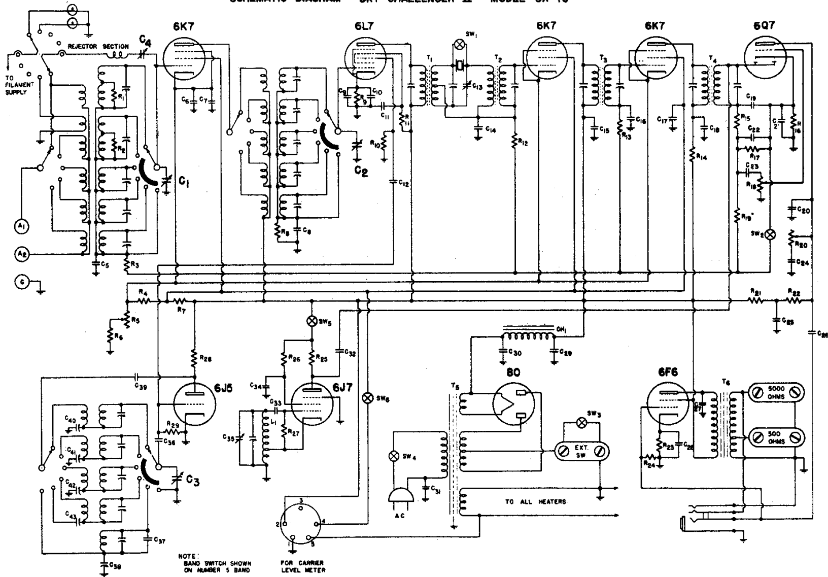
SCHEMATIC DIAGRAM - SKY CHALLENGER II - MODEL SX-18
