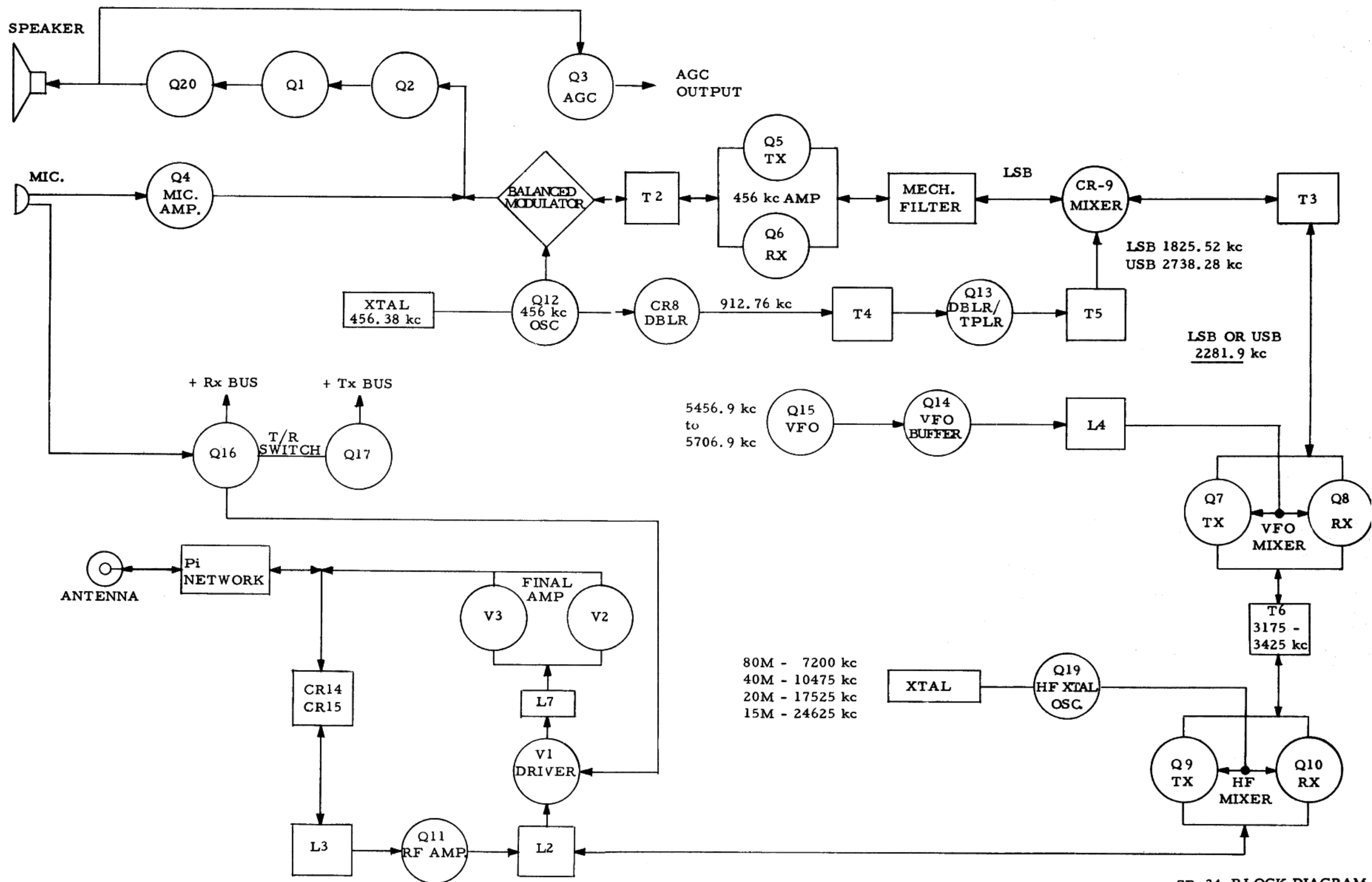
SB-34 BLOCK DIAGRAM
